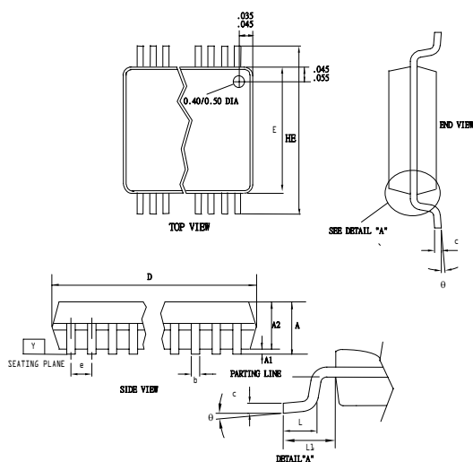
56 PIN SSOP-300mil
