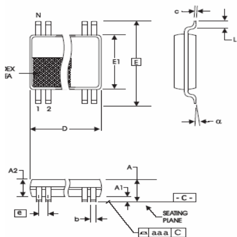
56 PIN TSSOP-240mil
